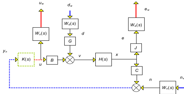
Fig. 7 Weighted block diagram for the beam problem
