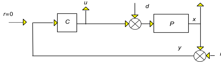
Fig. 3 Classical control block diagram
