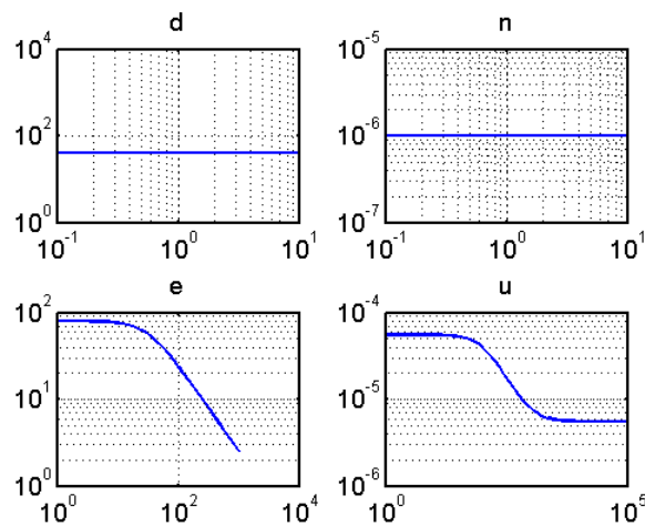
Fig. 15 Bode diagram
