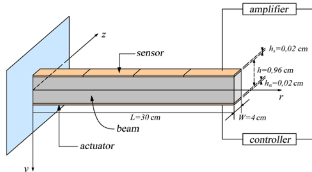
Fig. 1 Smart beam
