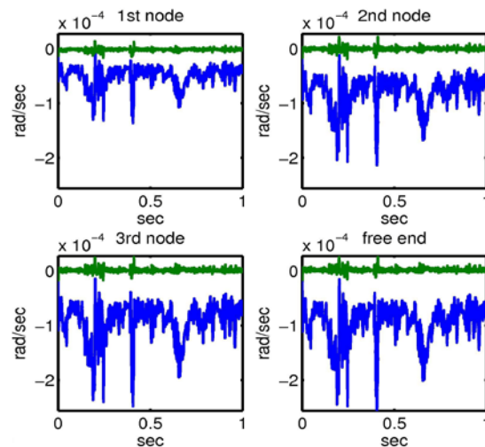
Fig. 12 Rotations of the four nodes of the beam without and with H_\infty control
