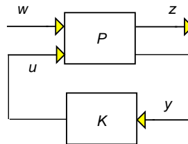
Fig. 5 Two-port diagram
