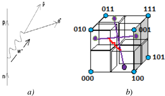
Fig. 6 a) The energy in this Feynman diagram is the given by E_{\text{output}} = W^- = -E , (negative boson in the field b_{\mu\nu}^a of mind (see the Theorem (1)). Then
