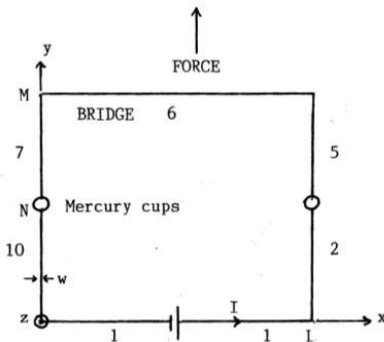
Fig. 1 Simplified model of Ampère's bridge
