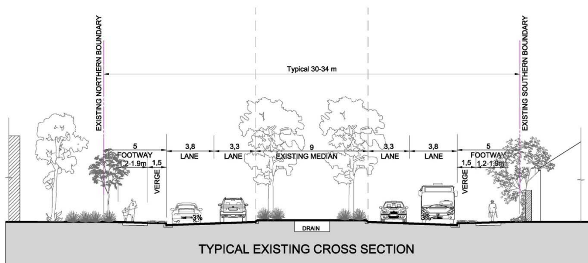
Fig. 1 Typical cross-section of Norwest Boulevard, Sydney, Australia
