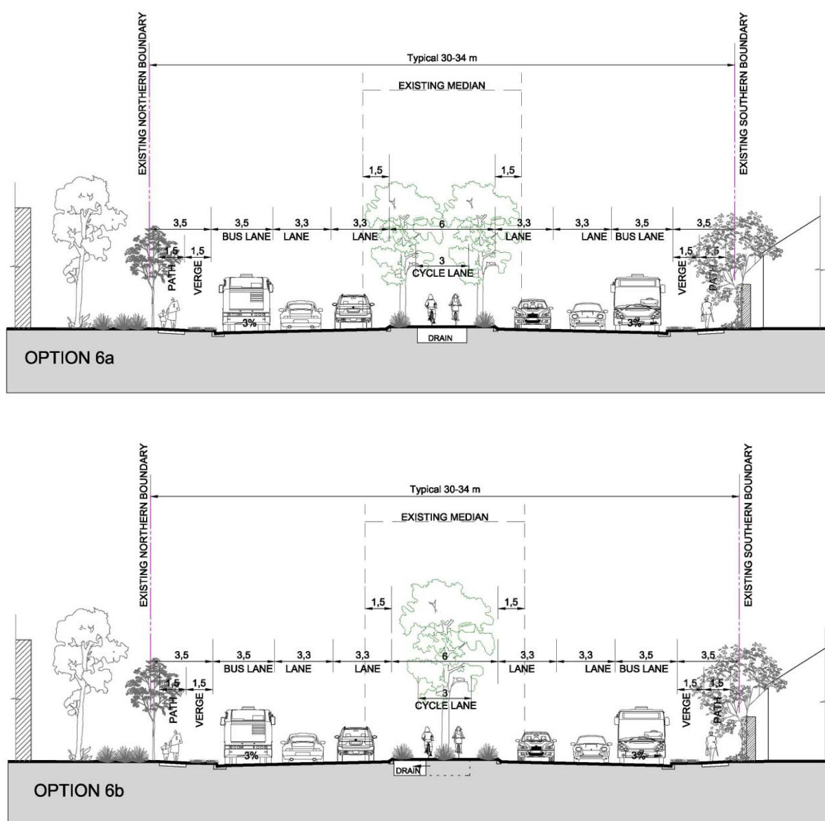
Fig. 3 Norwest Boulevard road corridor design options, in cross-section
