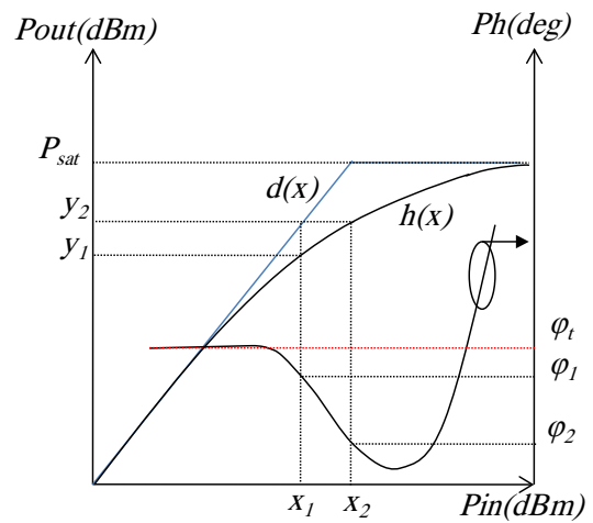
Figure 7 an example of AM/AM and AM/PM characteristics before and after linearization.(d(x) and \phi_t are characteristics of a linear PA)
