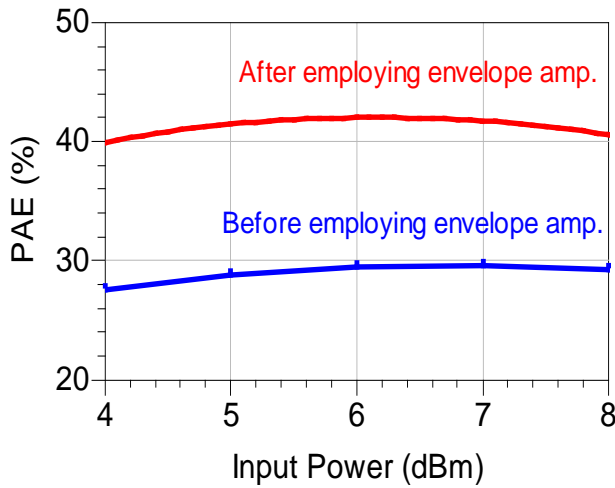
Figure 6 simulation of PA efficiency before and after employing envelope amplifier
