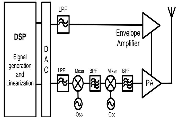
Figure 1 block diagram of lmds envelope tracking transmitter
