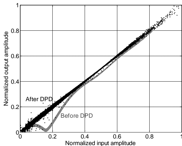
Figure 8 normalized AM/AM characterization of ET-PA before and after digital predistortion
