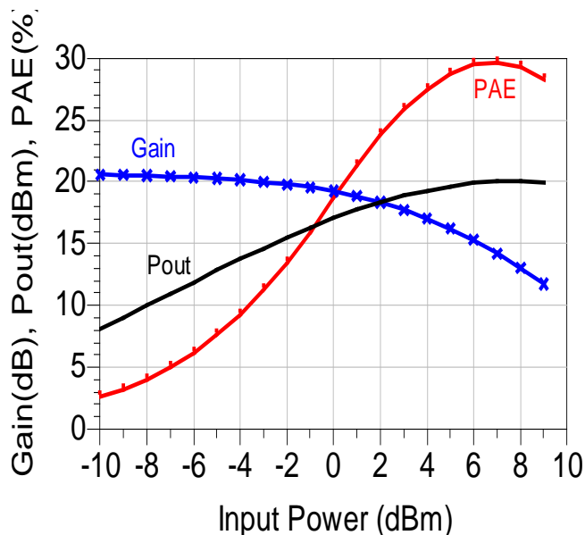
Figure 3 simulation results of 28 GHz PA gain, pout and PAE versus input power
