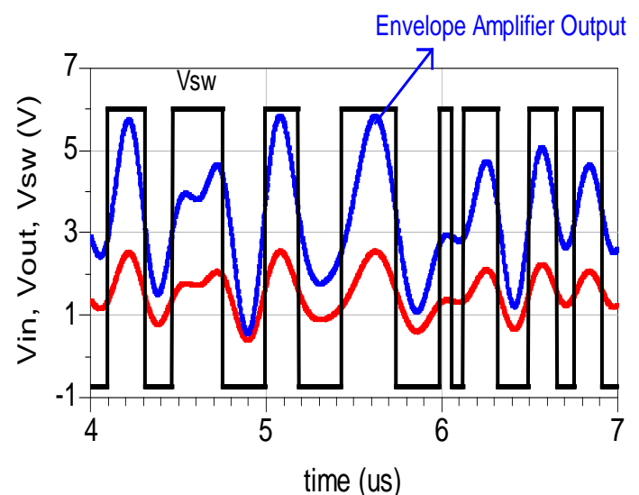
Figure 5 simulation of input and output voltages of envelope amplifier along with switching voltage.
