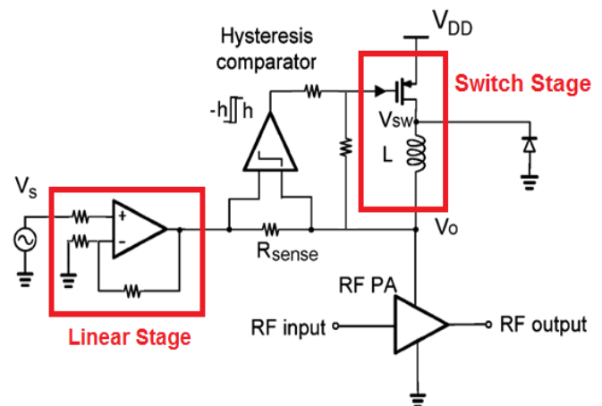
Figure 4 high efficient envelope amplifier [13]
