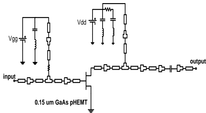
Figure 2 schematic of single stage GaAs pHEMT PA at 28 GHz
