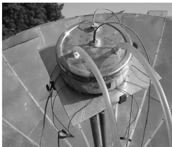
Figure 1 The arrangement of TEG setup
