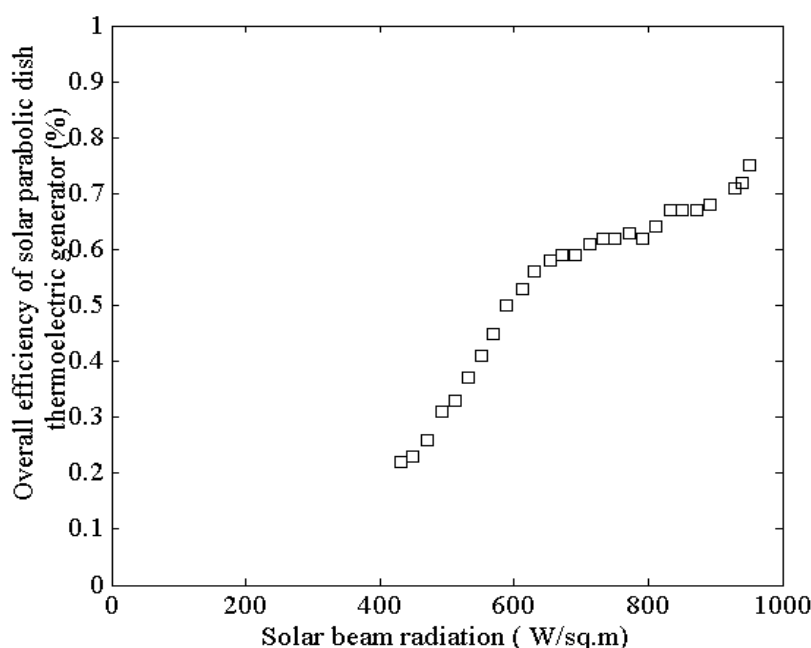
Figure 4 Overall efficiency of solar parabolic dish thermoelectric generator as function of solar beam radiation
