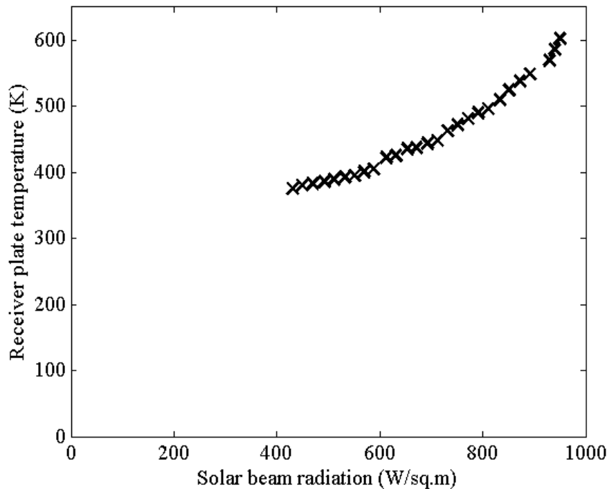
Figure 2 Receiver plate temperatures as function of solar beam radiation
