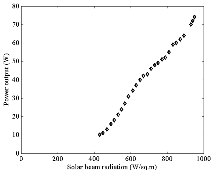
Figure 3 Maximum power output as function of solar beam radiation
