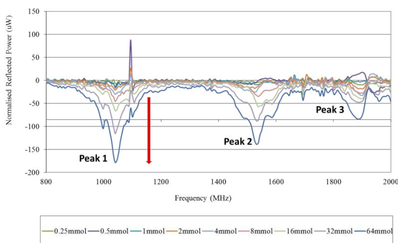
Fig. 3 Experimental spectra from 800-2000 MHz, shown as a normalised reflected power ( \mu W). The direction of the arrow indicates the increasing peak amplitudes with the increasing lactate acid concentration.
